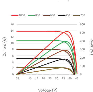
Characteristic Curves (515W)
