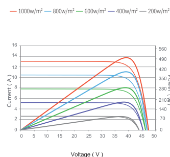
Current-Voltage & Power-Voltage Curves (505W)
