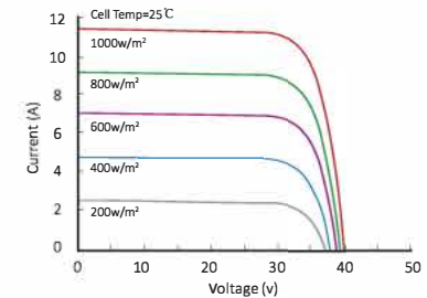
Current-Voltage Curve (LR4-60HPH-370M)
